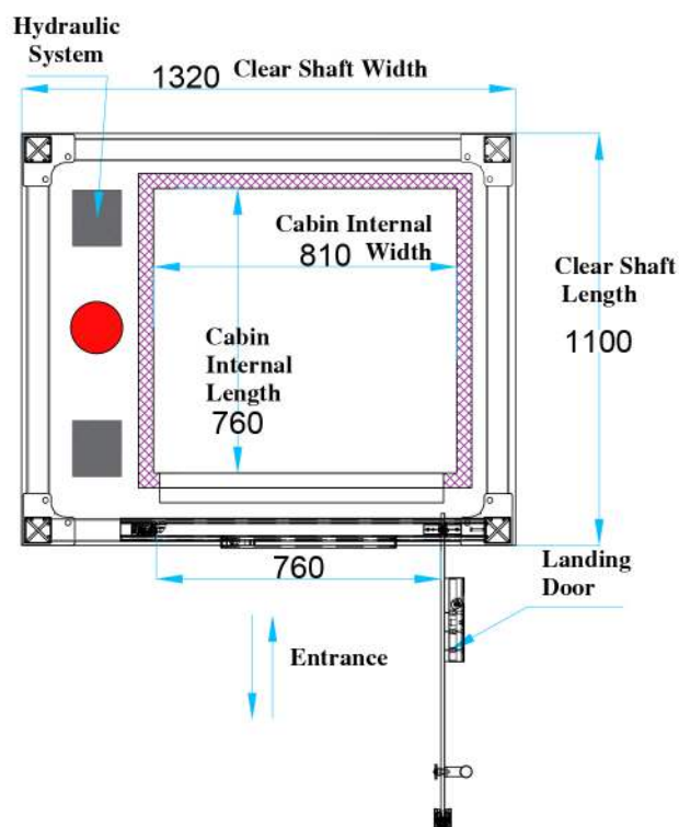
H250T Mini Elevator in Tower
