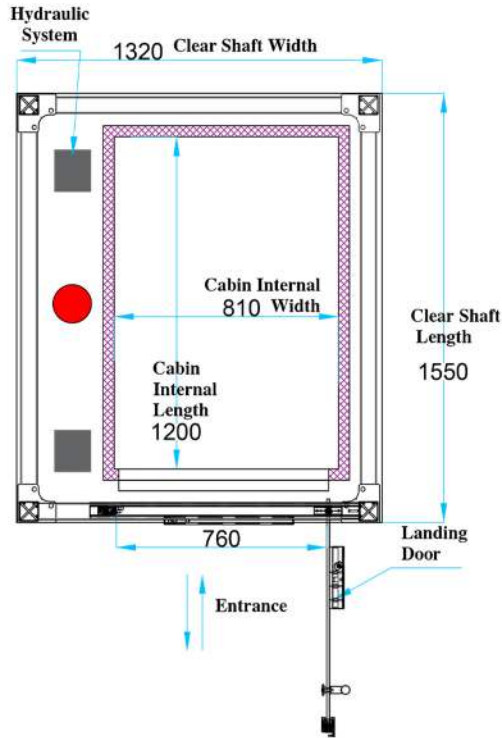
H250T Mini Elevator in Tower
